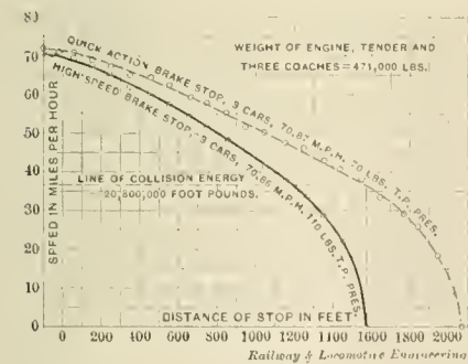
FIG. 5. COMPARATIVE 70 MILES PER HOUR STOPS.
